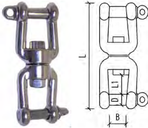
SWIVEL JAW AND JAW
