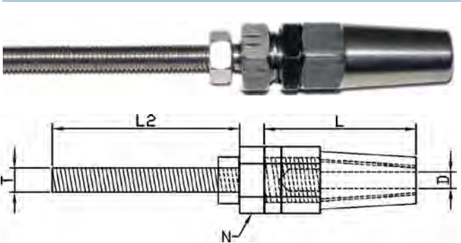
BRIDCO SWAGELESS TERMINAL
