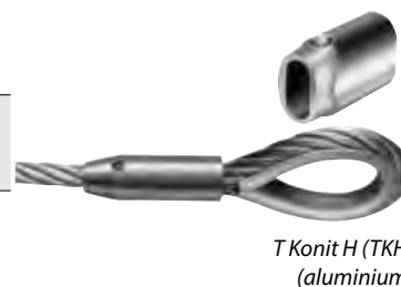
T Konit (TK) (aluminium)
