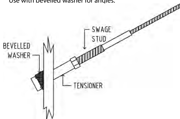
STAINLESS STEEL BEVELED WASHERS
