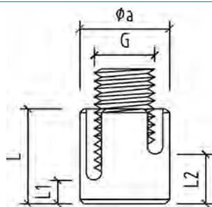
STAINLESS STEEL NET CLIP
