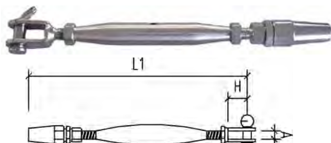
BRIDCO BOTTLESCREW JAW-SWAGELESS
