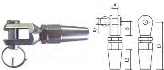
BRIDCO BOTTLESCREW FORK TERMINAL
