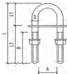
U BOLT - 304 GRADE
