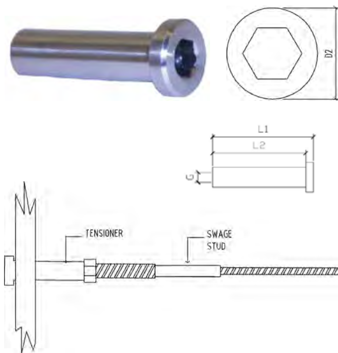
TENSIONER ALLEN KEY HEAD
