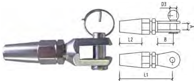
BRIDCO SWAGELESS FORK TERMINAL
